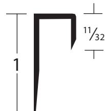
A-604S* 3/32" MAT'L MFA
