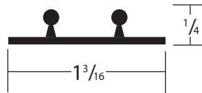
DOUBLE TRACK ACI-34
