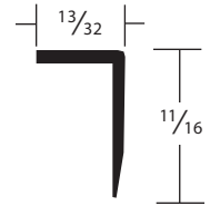
ACI 30 END CAP Stocked in Brite
