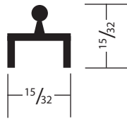
SINGLE TRACK ACI-38
