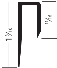
ACI-15 5/16" OPENING Stocked in Brite, Brushed Nickel, Matte Black, Polished Black, BREA & Oil Rub Bronze
