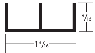
TOP CHANNEL ACI-33
