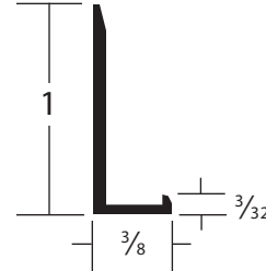
ACI 51 LITTLE LIP Stocked in Brite
