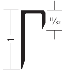
ACI-21 5/16" OPENING Stocked in Brite, Brushed Nickel, BREA, Polished Black & Oil Rub Bronze
