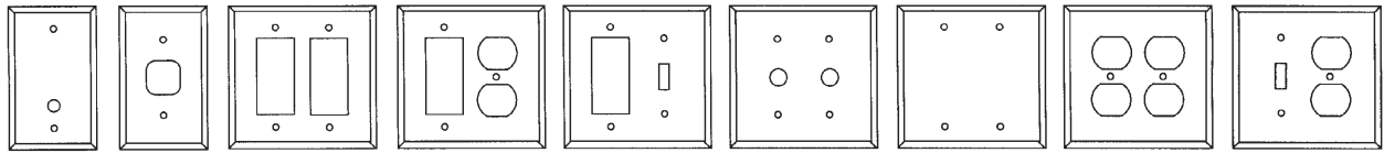
111 Single T.V.OFFSET (3/8") Hole 112 Single PHONE (Square) 202 Double DECORA 205 DECORA DUPLEX 206 DECORA TOGGLE 207 DOUBLE DIMMER 208 DOUBLE BLANK B-6 DOUBLE DUPLEX C-7 SWITCH DUPLEX
