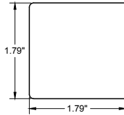
1 3/4" x 1 3/4" Clamp for 3/8" Glass (3.5mm walls)
