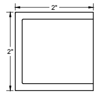
2" x 2" Clamp for 3/8" or 1/2" Glass (4.5mm walls)
