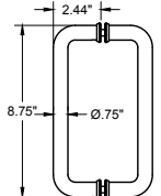
8" Back-to-Back Pull with removable washer
