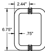
6" Back-to-Back Pull with removable washer
