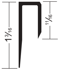
ACI-15 5/16" OPENING
